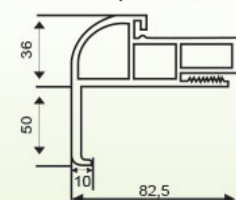
70 frame profile with fixed border
